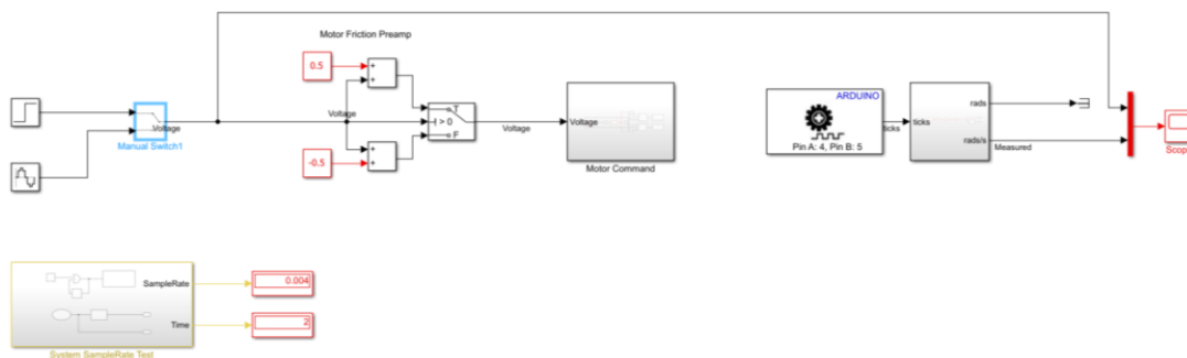
Figure 10 Simulink model : HexaMotor_System_Identification_V02.slx ”
